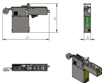
Tape adjustment feeder(GS-RAZ2211) Schematic diagram of appearance and dimensions (Unit :mm)
